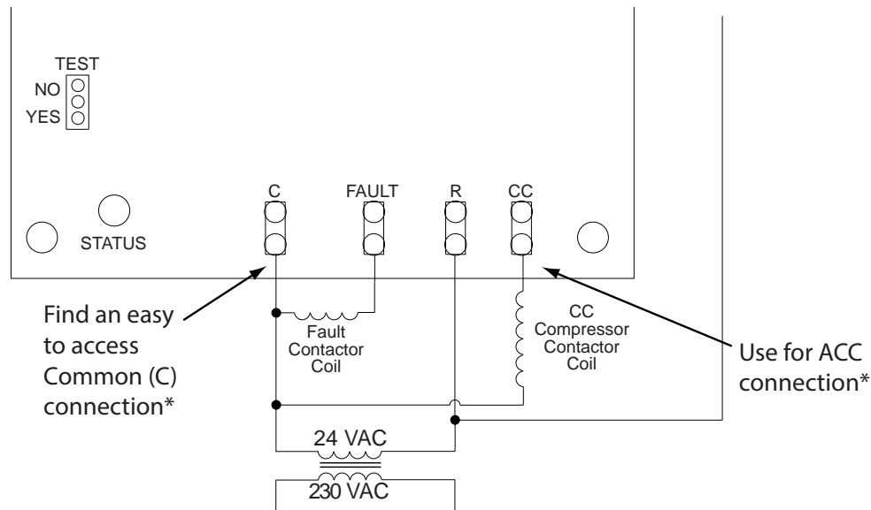
Figure 6: Connections for heat pumps with an external compressor contactor, but without an accessory relay
