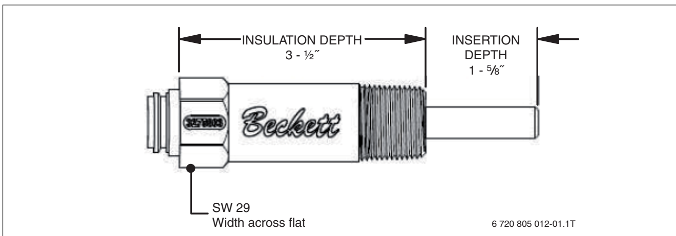
Fig. 2 Sensor well
