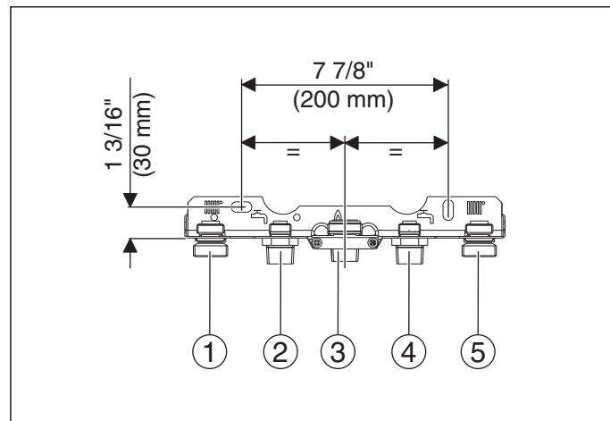
Figure 3 Correct hydraulic connection plate dimensions
